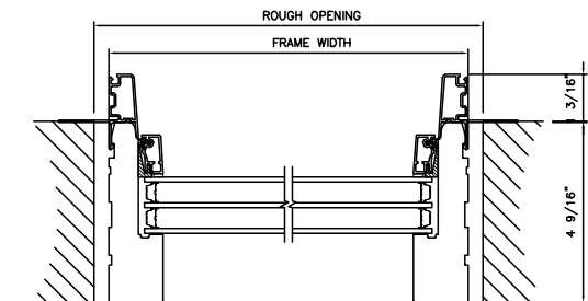
METAL CLAD TRIPLE PICTURE 4 9/16" (116mm)
