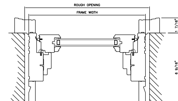
WOOD EXTERIOR DOUBLE CASEMENT 9/16" (166mm)
