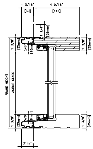
METAL CLAD PICTURE (DUAL GLAZED) 4 9/16" (116mm)
