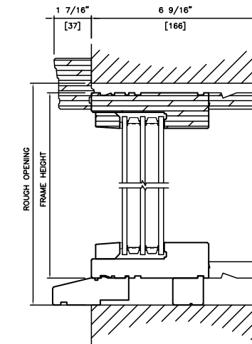
WOOD EXTERIOR TRIPLE PICTURE 6 9/16" (166mm)
