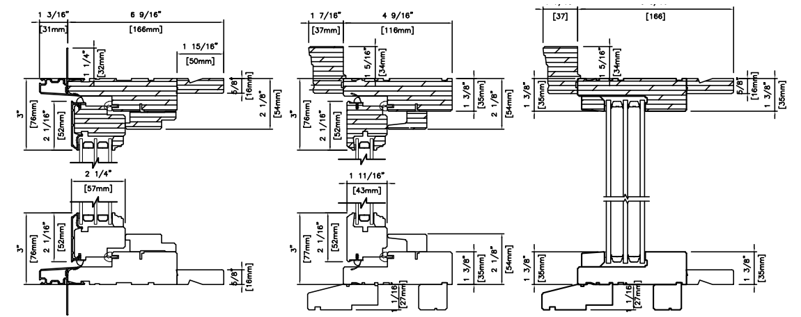
METAL CLAD CASEMENT (TRIPLE GLAZED) 6 9/16" (166mm) ROTOGEAR MOULDINGS
