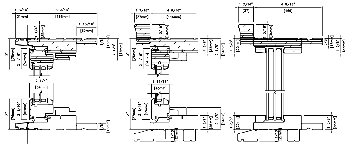
METAL CLAD CASEMENT (TRIPLE GLAZED) 6 9/16" (166mm) ROTOGEAR MOULDINGS
