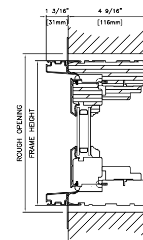
METAL CLAD DOUBLE CASEMENT 4 9/16" (116mm)
